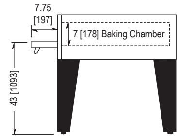
SIDE VIEW - EDO 2136 Single
