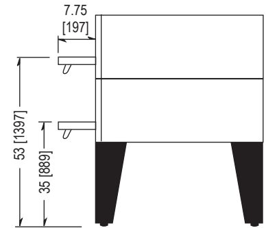
SIDE VIEW - EDO 2136 Double
