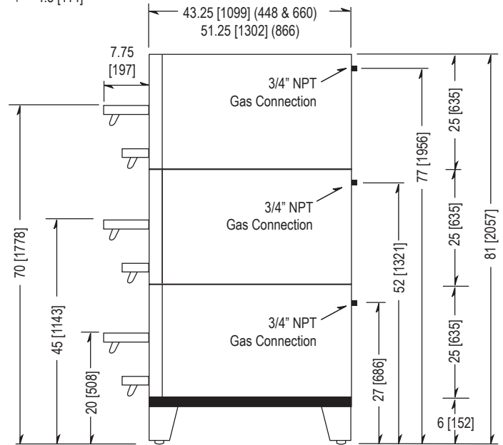
SIDE VIEW STACKED SD 448/660/866
