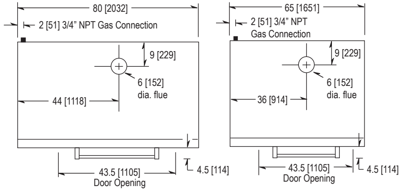
TOP VIEW SD 660
